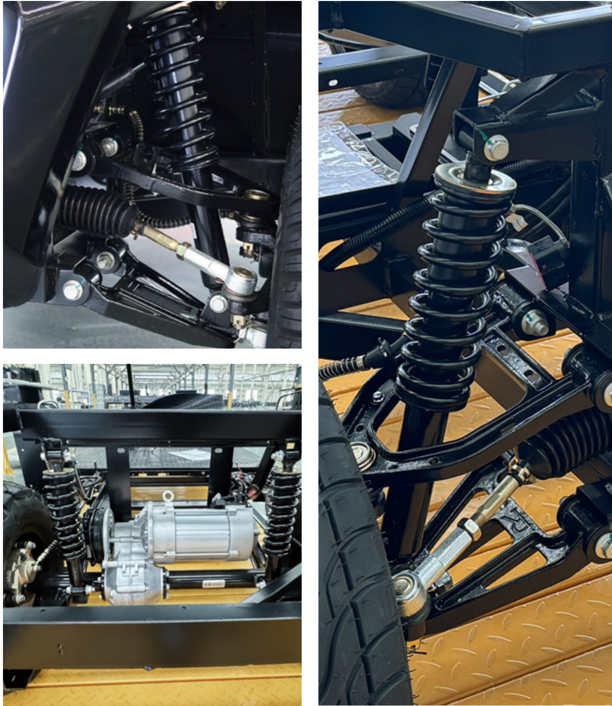
Coilover Suspension With Extra Springs For A Smooth Ride
